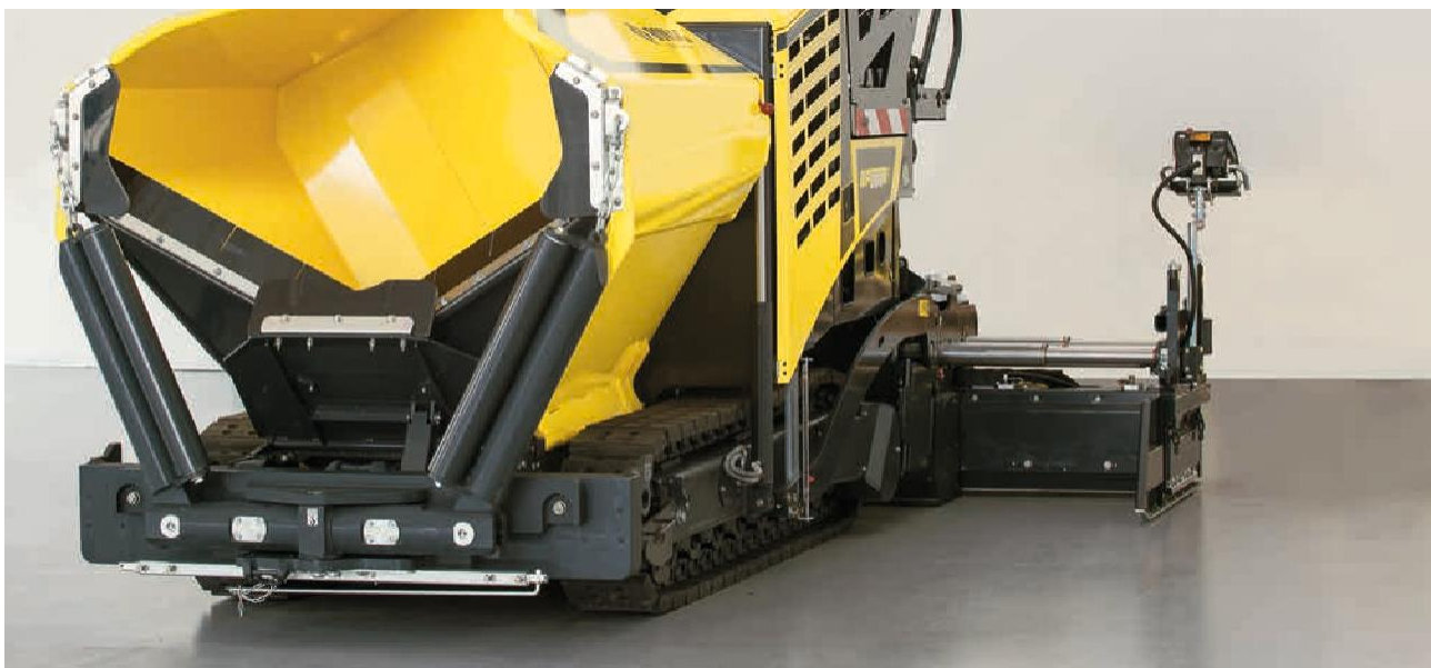
Optional hydraulic hopper wing.
